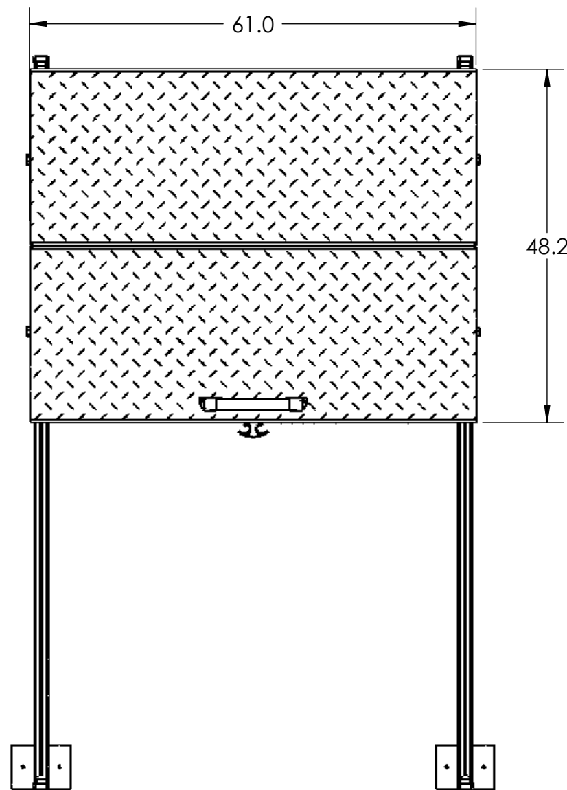
TOP VIEW
