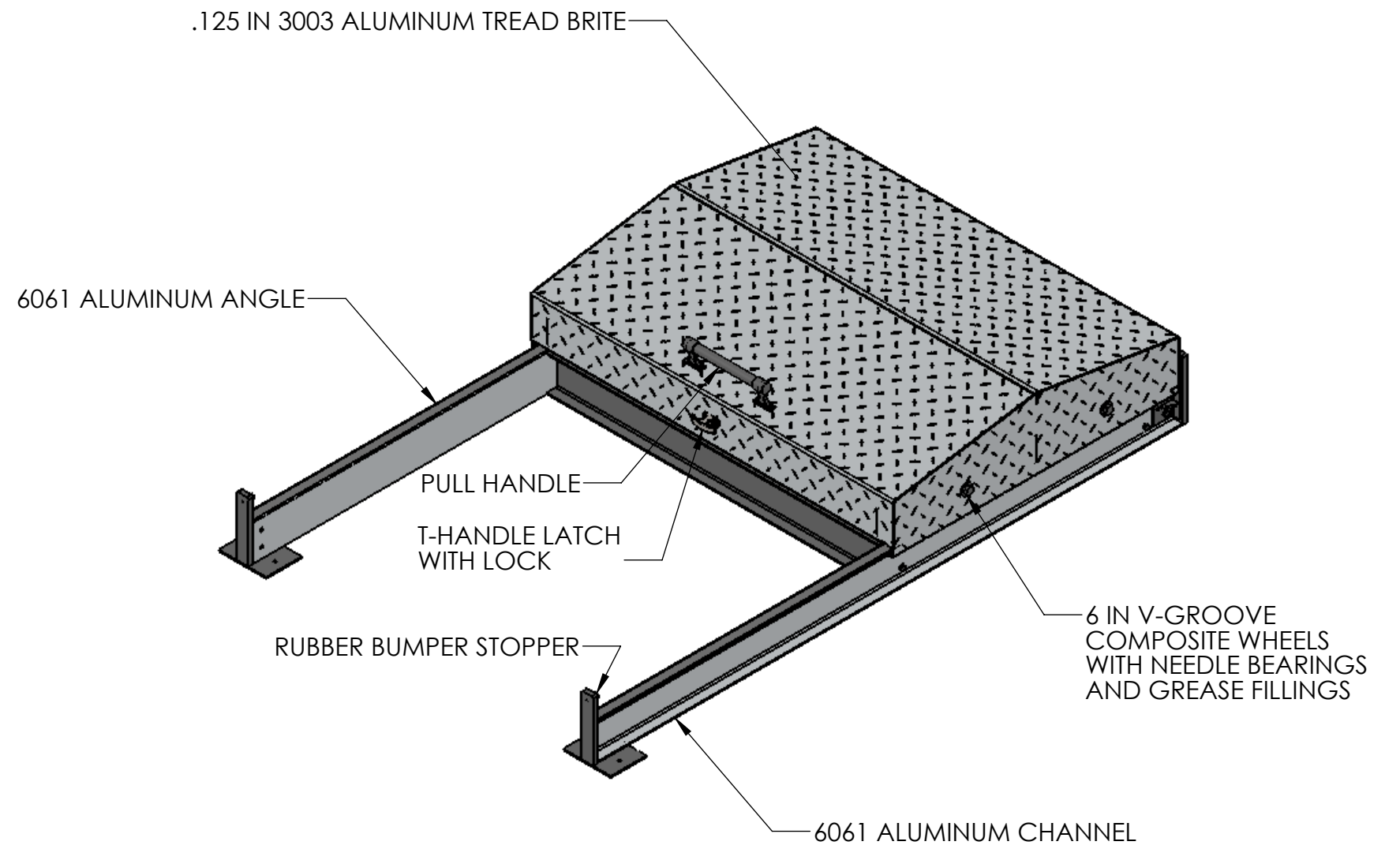
ISOMETRIC VIEW
