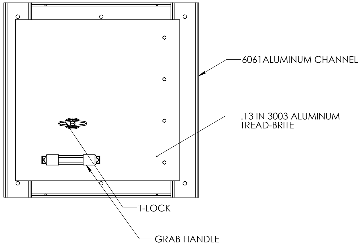
TOP VIEW
