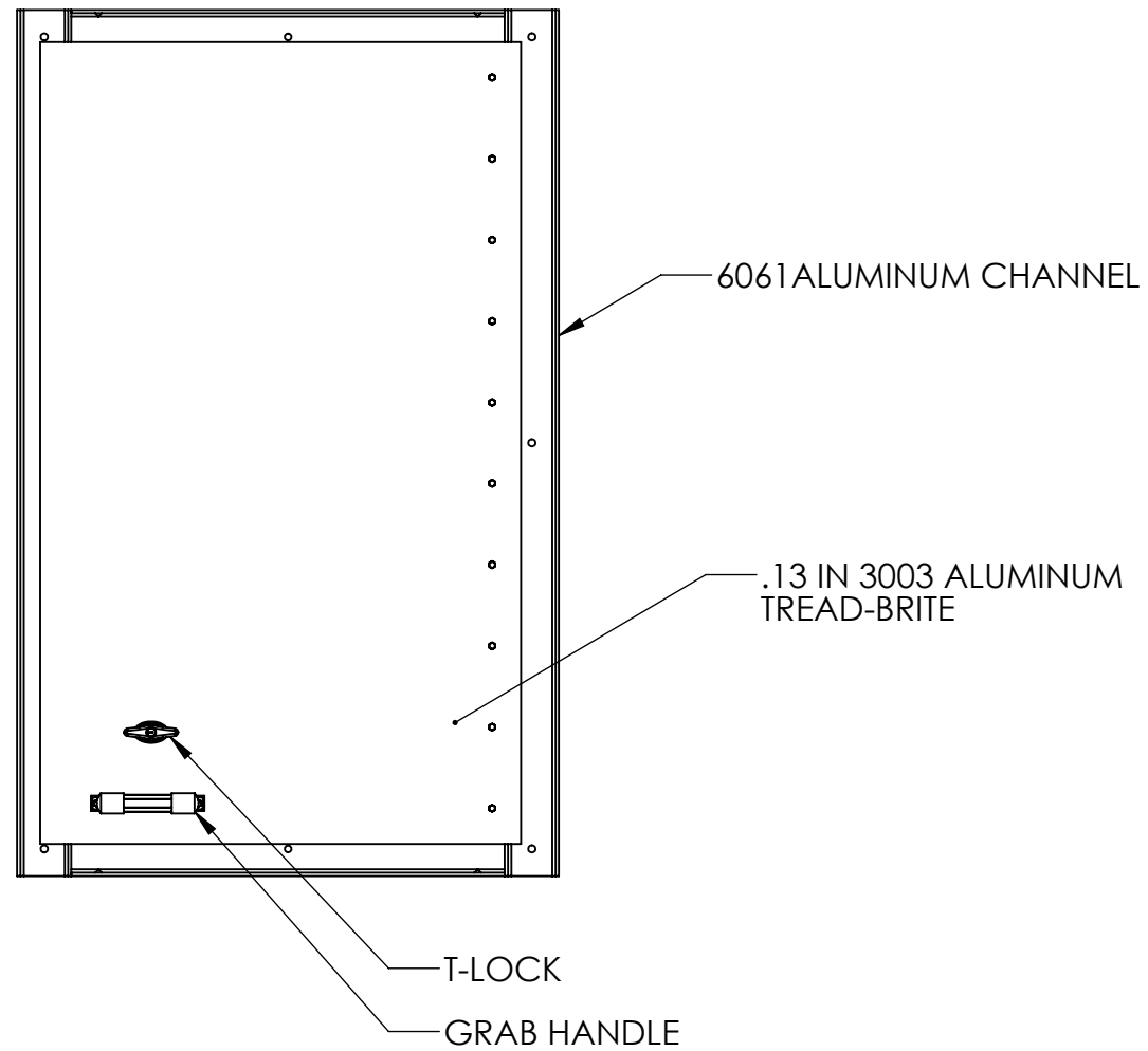
TOP VIEW
