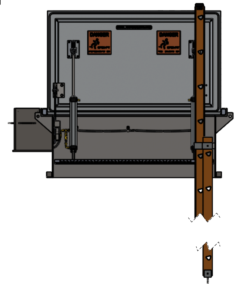
FRONT CUT VIEW
